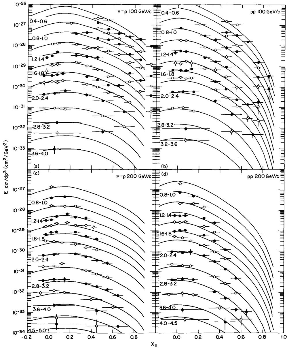
Fig. 1. The invariant cross section for \pi^0 production versus x_{||} for several reactions: (a) \pi^-p at 100 GeV/c; (b) pp at 100 GeV/c; (c) \pi^-p at 200 GeV/c; (d) pp at 200 GeV/c. For display purposes, the cross sections in alternate p_{\perp} intervals are labelled. Smooth curves indicate the parametrization described in the text.
