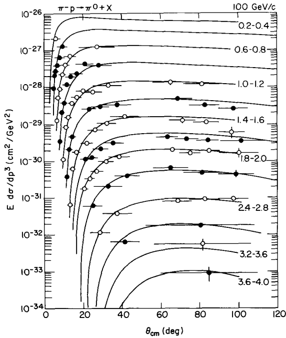
Fig. 2. The invariant cross section versus \theta_{cm} for \pi^-p \rightarrow \pi^0 + X at 100 GeV/c. Alternating p_\perp intervals are labelled and are denoted by open and closed symbols. These points are plotted at the \theta_{cm} corresponding to the bin centers of p_\perp, x_\parallel bins shown in fig. 1a. The smooth curves display the parametrization described in the text.
