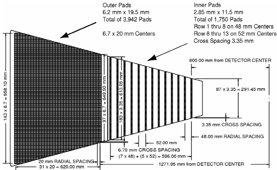
Fig. 4. The anode pad plane with one full sector shown. The inner sub-sector is on the right and it has small pads arranged in widely spaced rows. The outer sub-sector is on the left and it is densely packed with larger pads.
