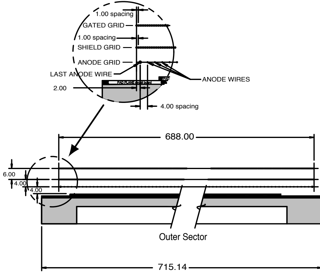
Fig. 3. A cutaway view of an outer sub-sector pad plane. The cut is taken along a radial line from the center of the TPC to the outer field cage so the center of the detector is towards the right hand side of the figure. The figures shows the spacing of the anode wires relative to the pad plane, the ground shield grid, and the gated grid. The bubble diagram shows additional detail about the wire spacing. The inner sub-sector pad plane has the same layout except the spacing around the anode plane is 2 mm instead of the 4 mm shown here. All dimensions are in millimeters.
