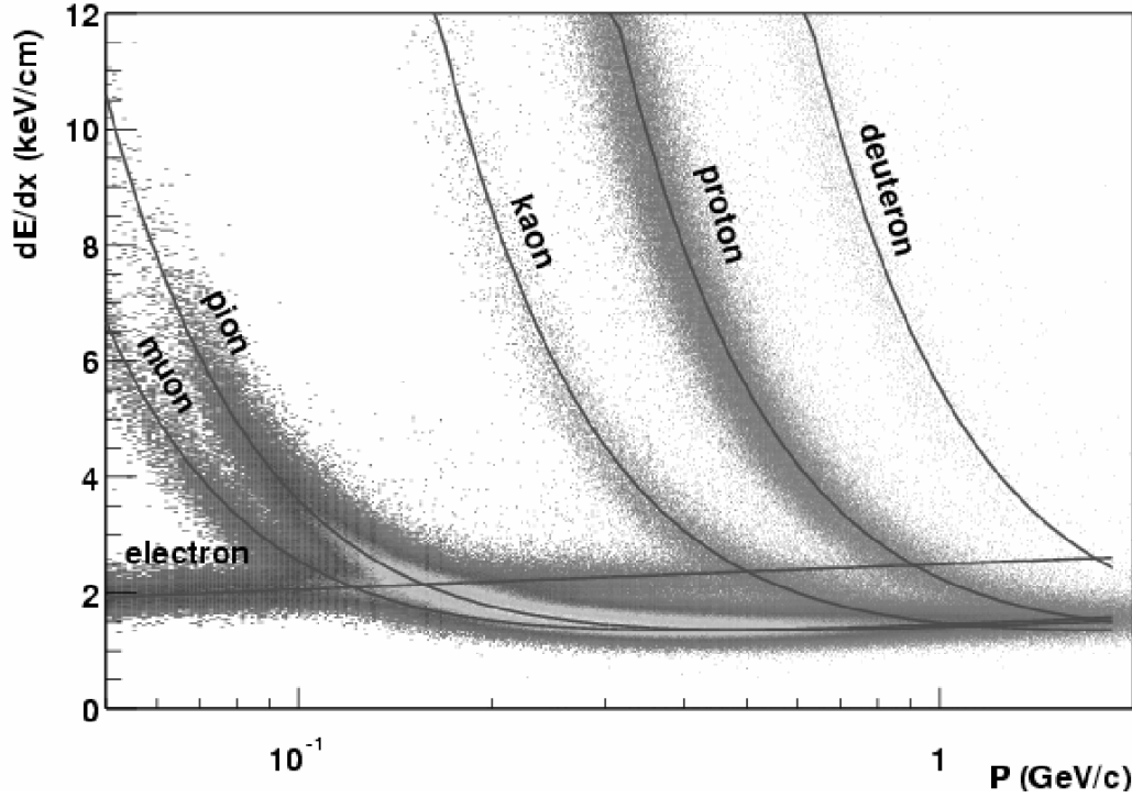
Fig. 11. The energy loss distribution for primary and secondary particles in the STAR TPC as a function of the p_T of the primary particle. The magnetic field was 0.25 T.
