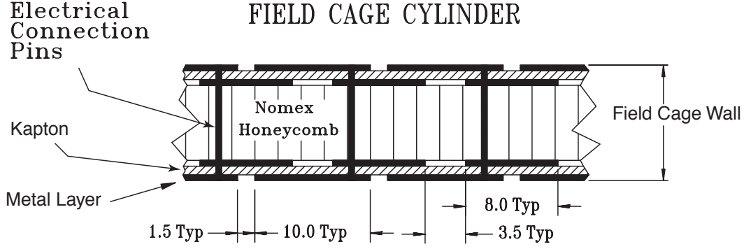
Fig. 2. A cutaway view of the inner field cage (IFC) showing the construction and composition of the cylinder wall. Dimensions are in mm.
