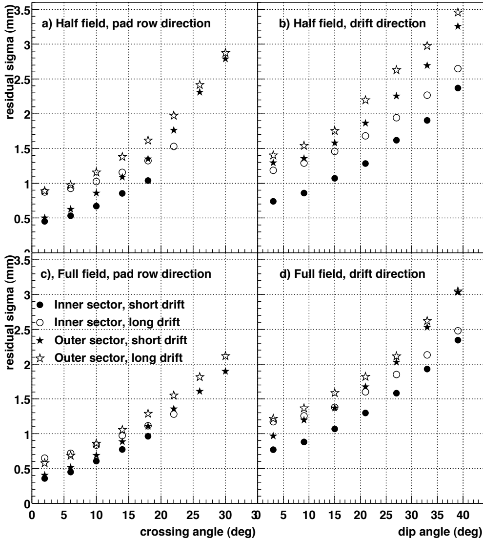
Fig. 5. Position resolution across the pad rows and along the z axis of the TPC. The crossing angle is the angle between the particle momentum and the pad row direction. The dip angle is the angle between the particle momentum and the drift direction, \theta = \cos^{-1}(p_z/p) .
