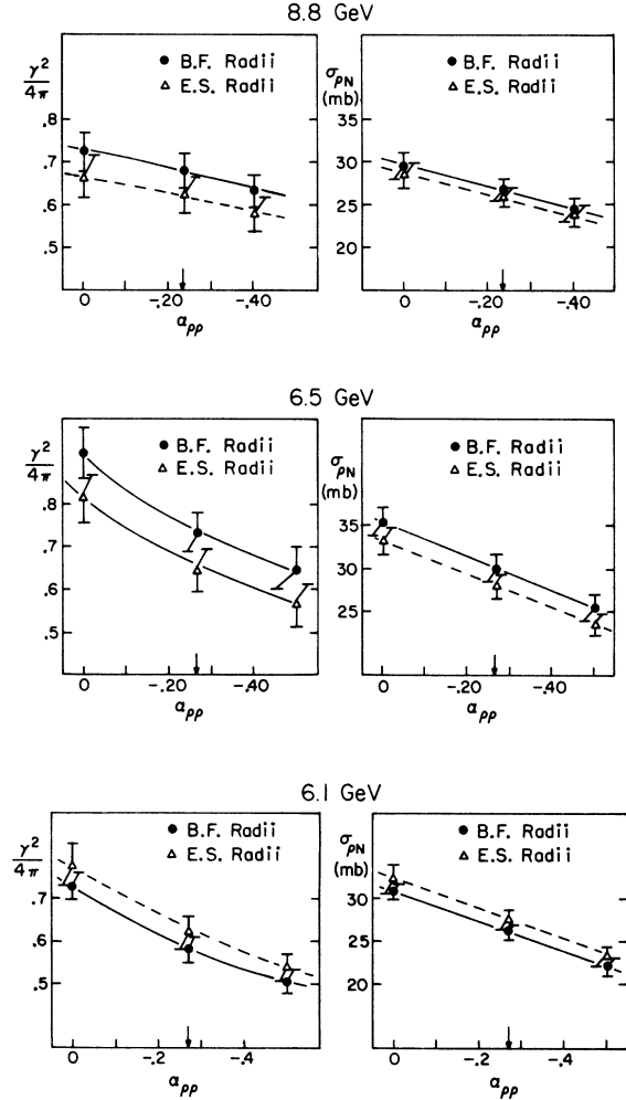
FIG. 7. Variation of the parameters \gamma_\rho^2/4\pi and \sigma_{\rho N} with \alpha_{\rho\rho} .
